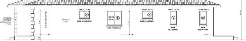
RIGHT SIDE (EAST) ELEVATION
