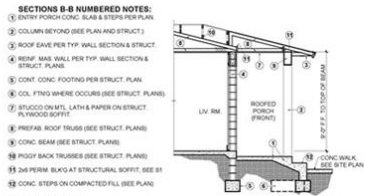
SECTION B-B CROSS SECTION THROUGH FRONT ROOFED PORCH FACING STREET
